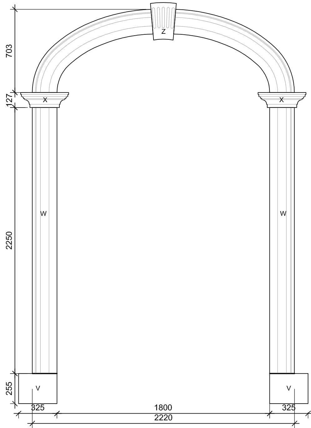
1800 ARCH DETAIL: Scale 1:20
