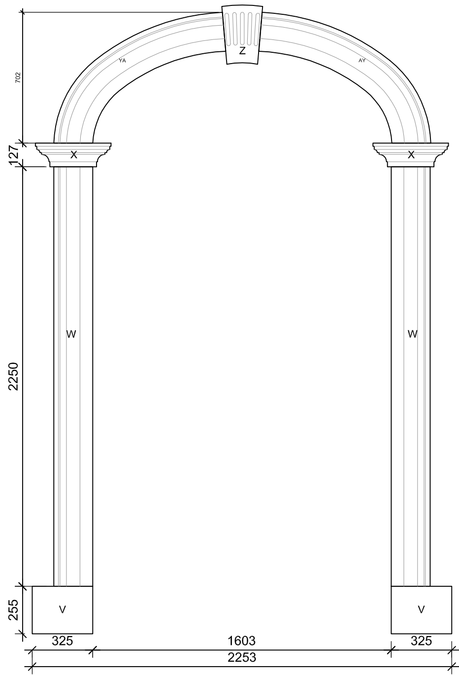
1600 ARCH DETAIL: Scale 1:20
