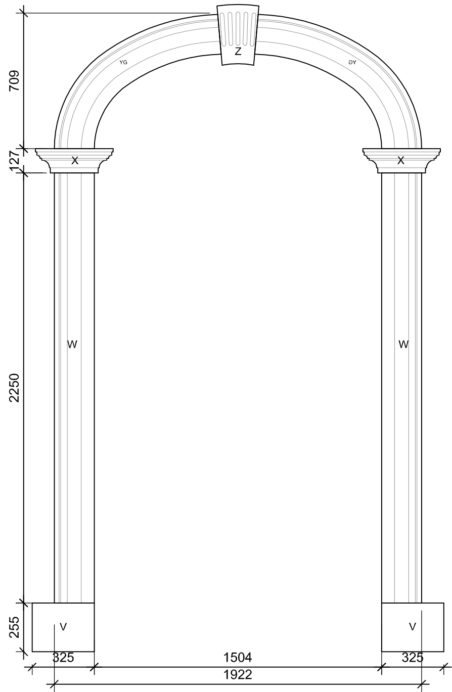
1500 ARCH DETAIL: Scale 1:20
