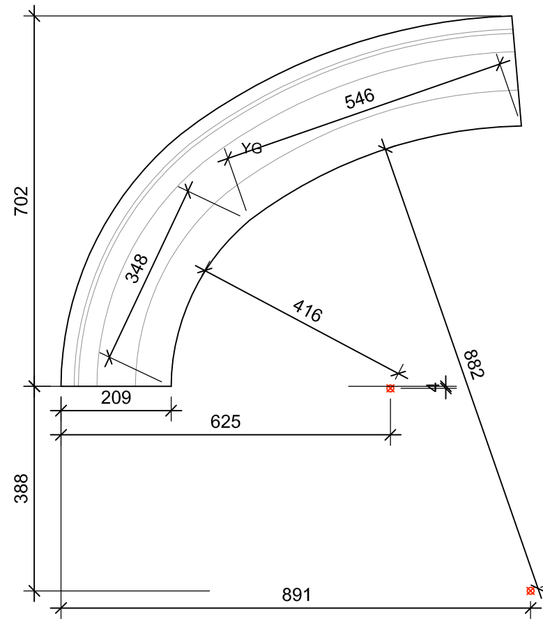
1500 ARCH DETAIL: Scale 1:10
