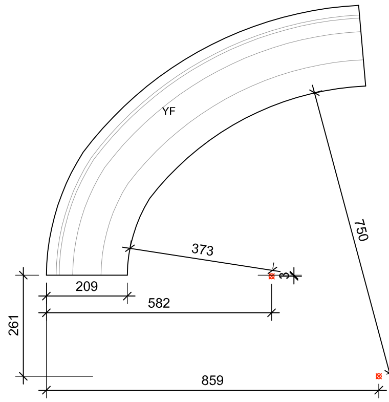
1400 ARCH DETAIL: Scale 1:10
