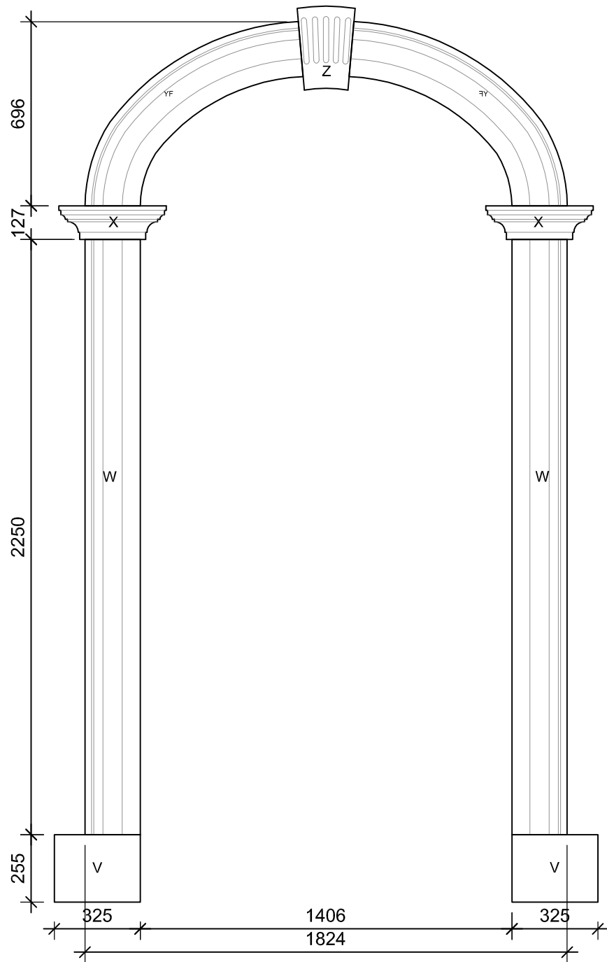
1400 ARCH DETAIL: Scale 1:20
