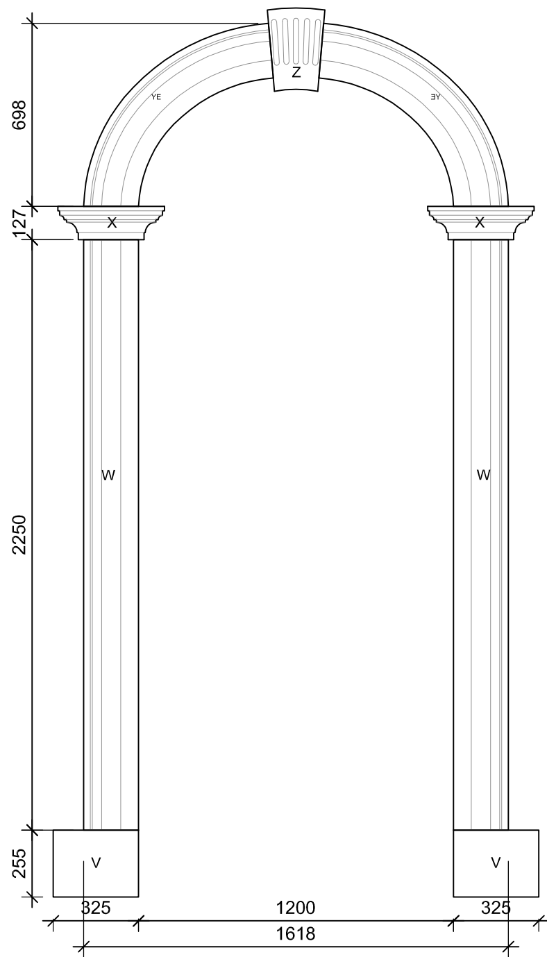
1200 ARCH DETAIL: Scale 1:20
