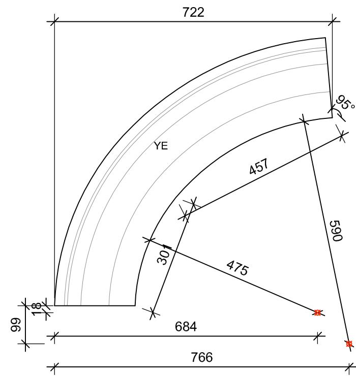
1200 ARCH DETAIL: Scale 1:10
